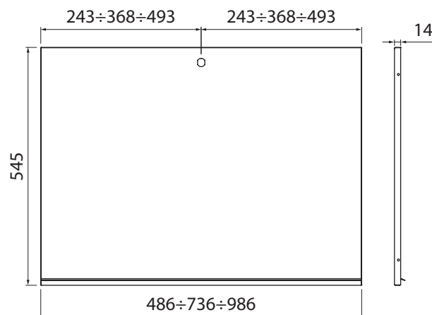
Porta per armadietto Slim Door for slim cabinet
